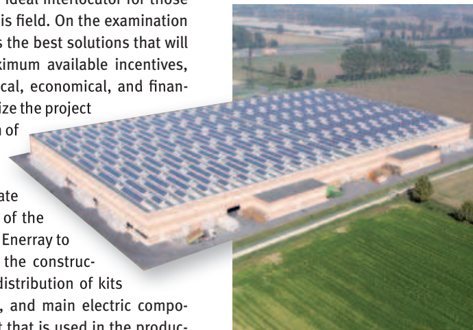
PV plant on a commercial roof (1.43 MWp) developed by Enerray in Martinego
